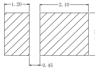
1-4 Soldering patterns 推荐焊盘
