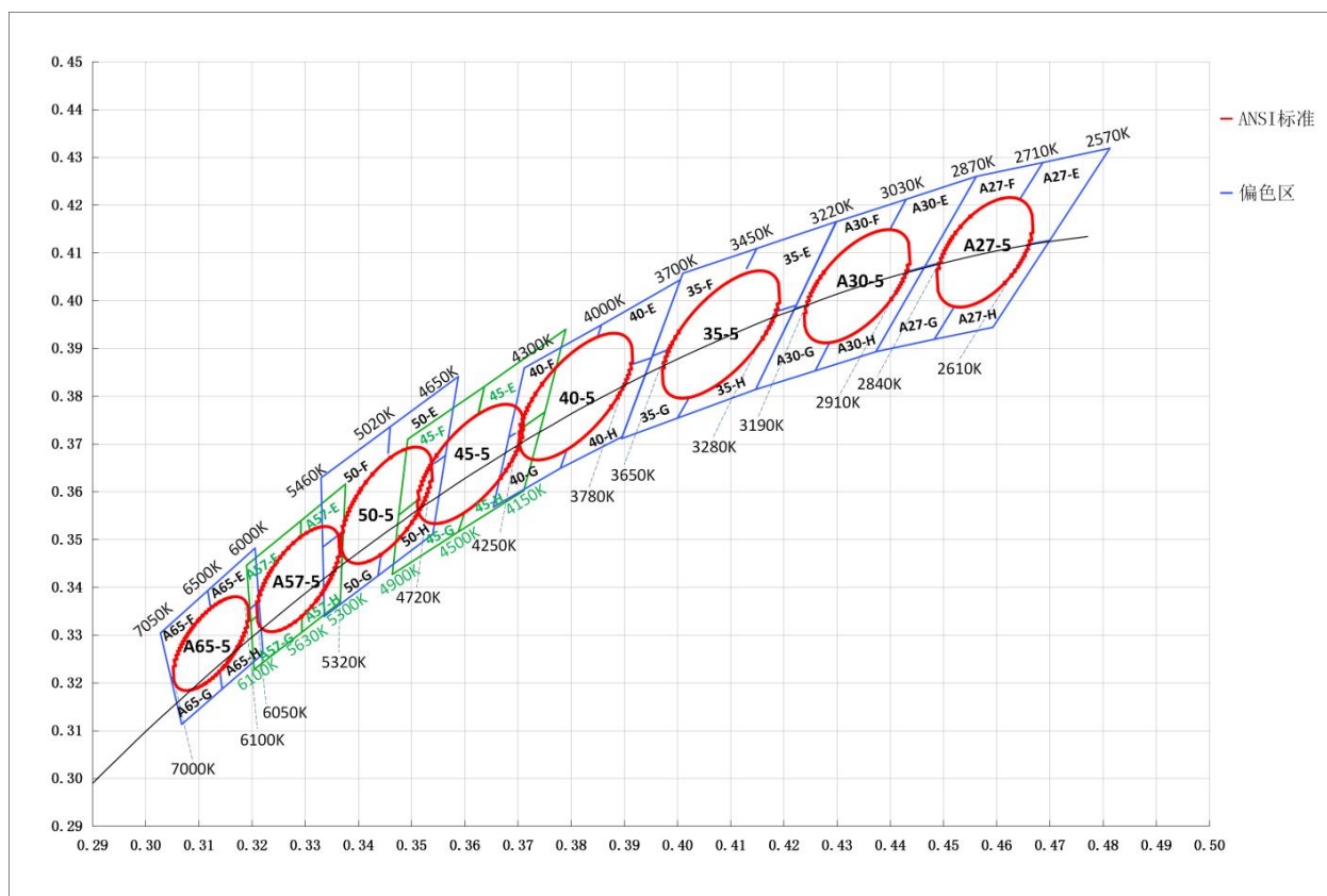
CIE Chromaticity Diagram @IF=30mA, T a =25℃ (色区图)
