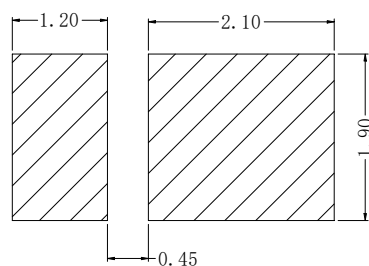
1-2 Side view 侧视图
