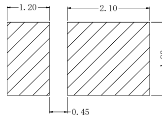
1-4 Soldering patterns 推荐焊盘
