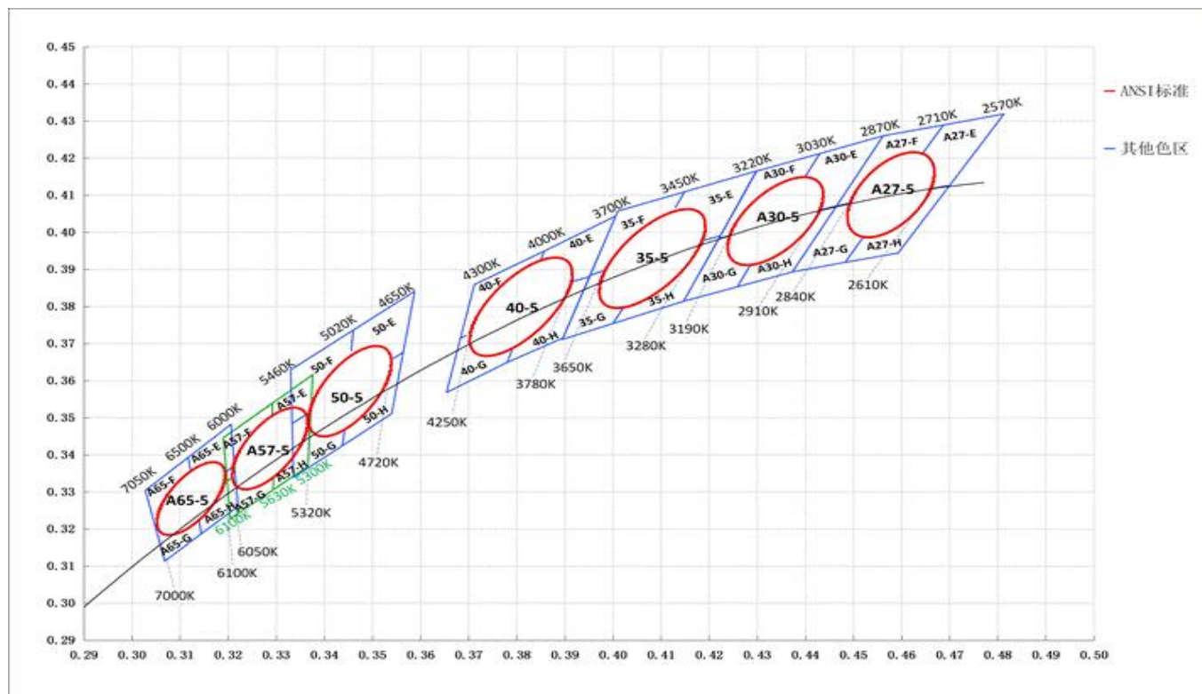
CIE Chromaticity Diagram @IF=60mA, T_a=25^\circ\text{C} (色区图)
