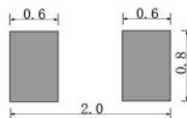
1-4 Soldering patterns推荐焊盘
