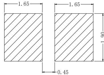
1-4 Soldering patterns 推荐焊盘
