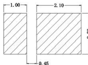
1-4 Soldering patterns 推荐焊盘
