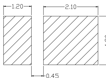
1-4 Soldering patterns 推荐焊盘
