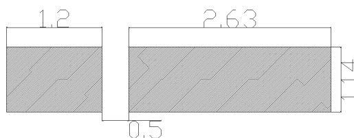
1-4 Soldering patterns 推荐焊盘
