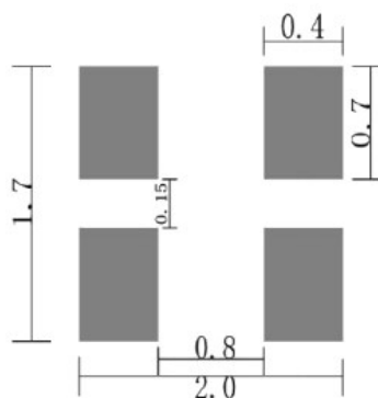
1-4 Soldering patterns 推荐焊盘
